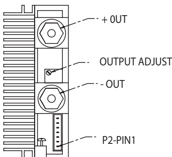
P2 REMOTE SENSE TRIM/SC & POWER GOOD
